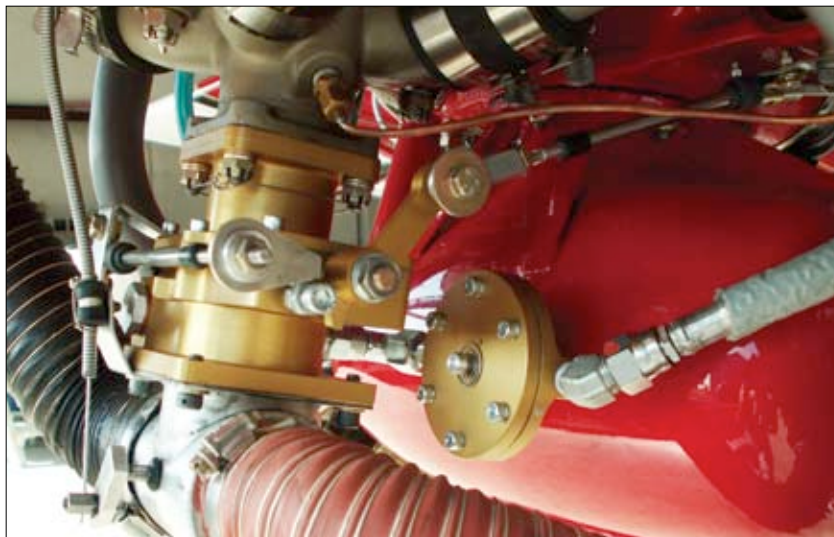
Mike Custard's O-200 TBI installation. The throttle slide is facing toward you; the gold disk next to the engine sump is the pressure regulator.
