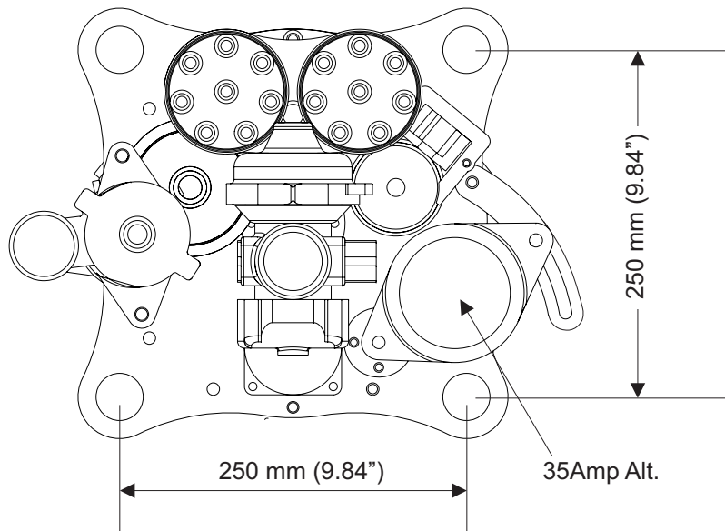
VIEW OF REAR MOUNTING PLATE AND BOLT ON ACC'S
